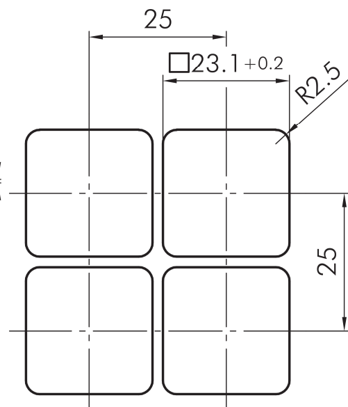
Drilling pattern
