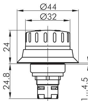
Dimensional drawing
