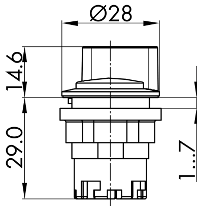
→ Dimensional drawing
