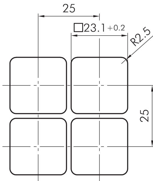
Drilling pattern
