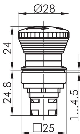
Dimensional drawing
