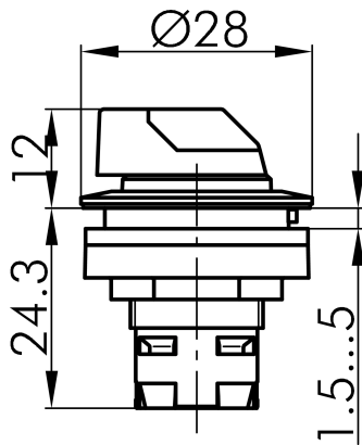
→ Dimensional drawing
