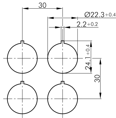
→ Cutout dimensions
