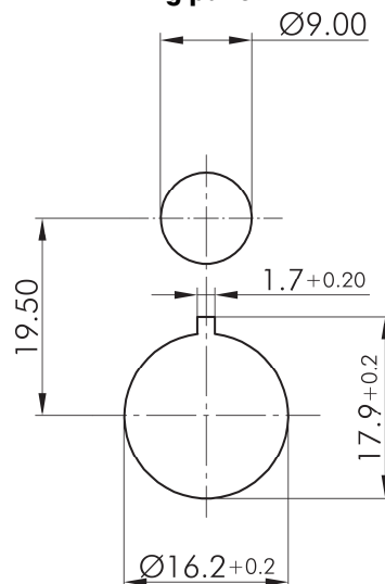
Drilling pattern
