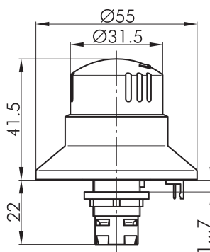
Dimensional drawing
