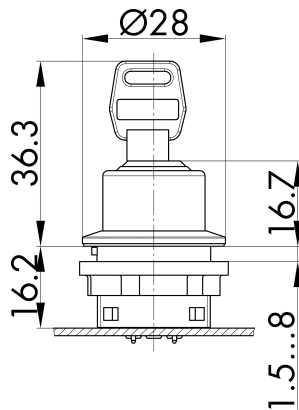
→ Dimensional drawing
