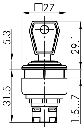
→ Dimensional drawing
