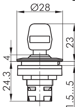
Dimensional drawing
