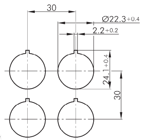
Drilling pattern
