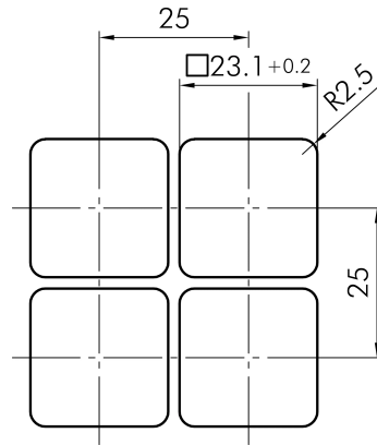
→ Cutout dimensions
