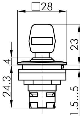
→ Dimensional drawing
