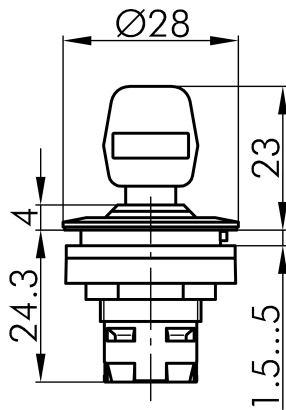
→ Dimensional drawing
